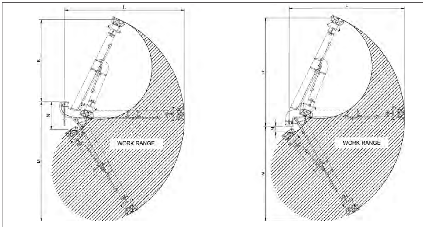
YOGA - Extraction arms reach dimensions
