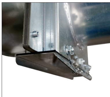
Discharge lid on the underside of the damper
